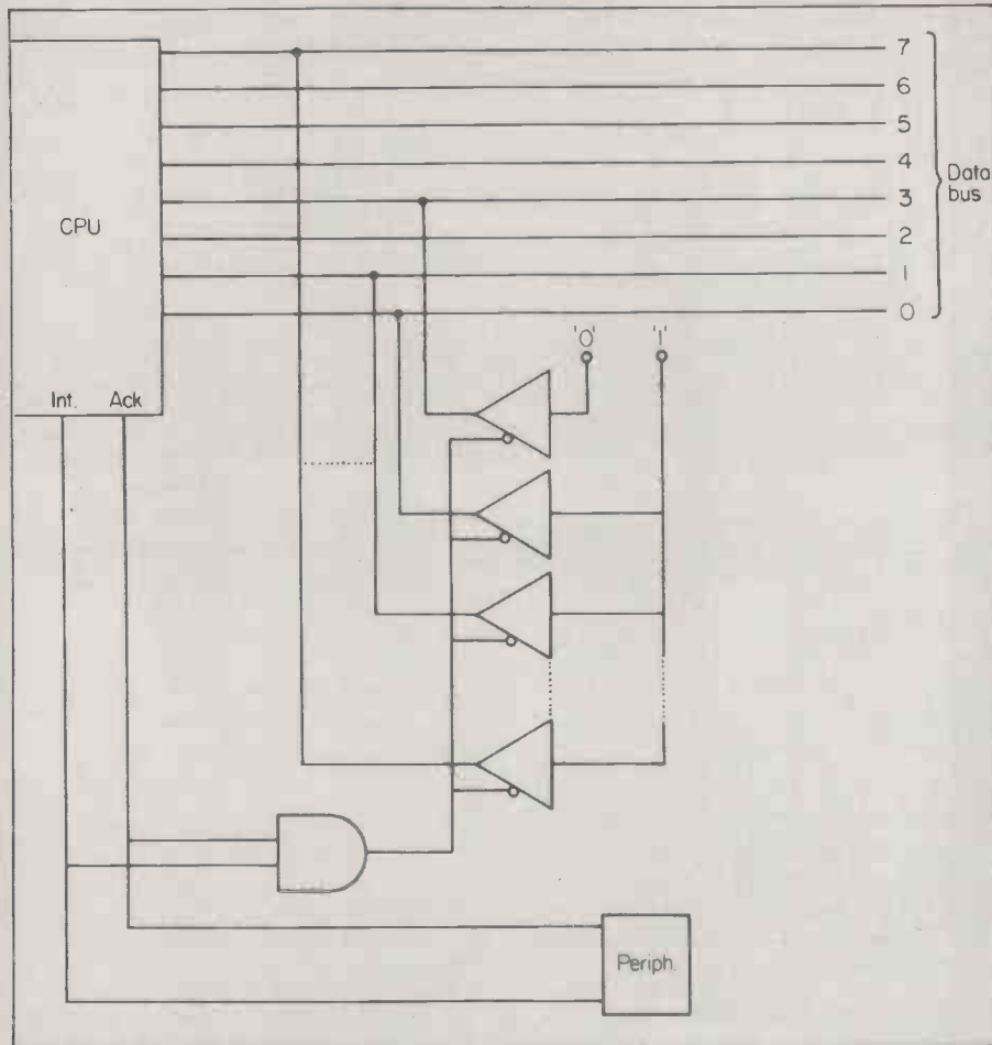
Figure 9. Hard-wired 'RST30'.
